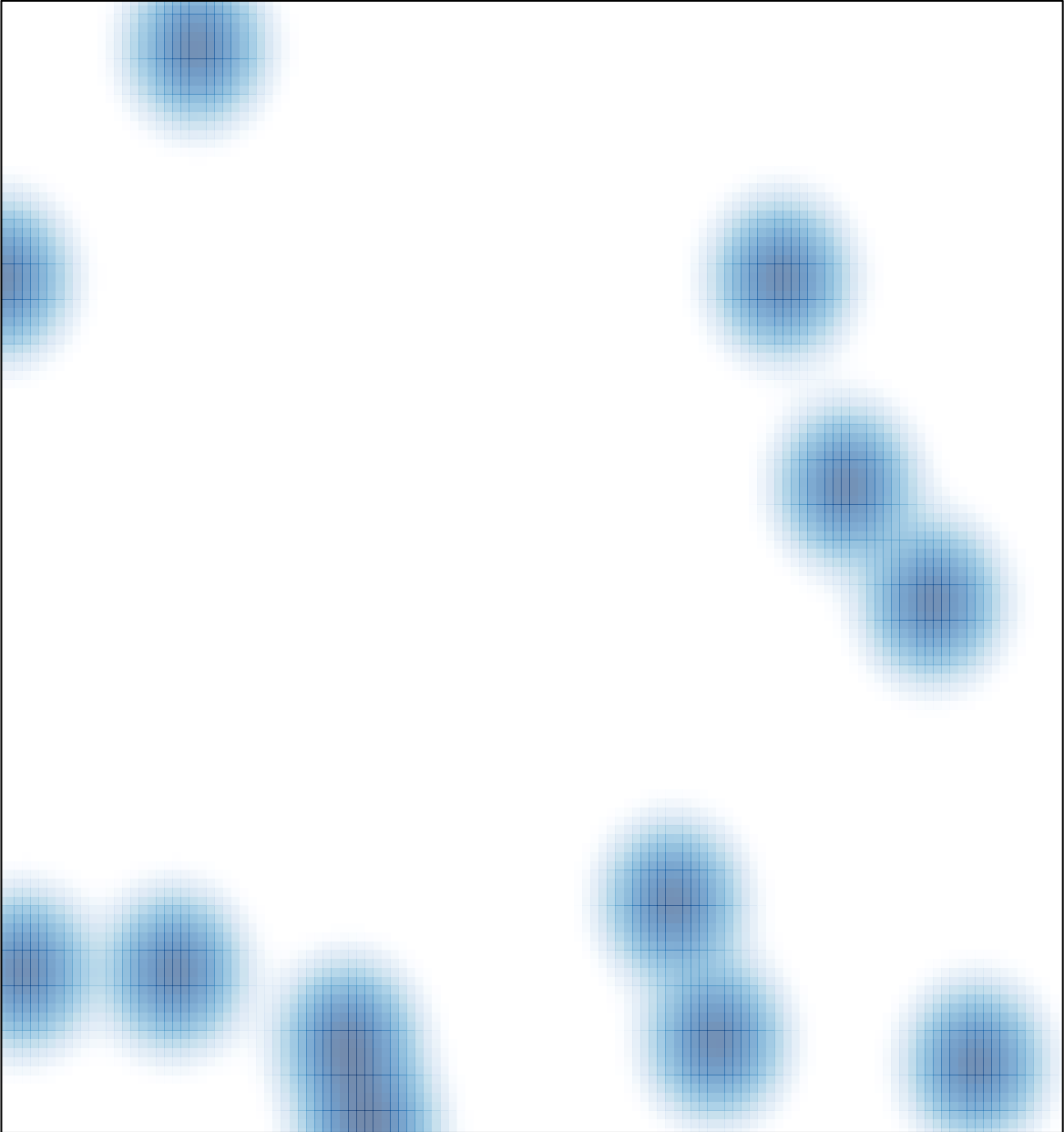
# features = 13 , max = 1
